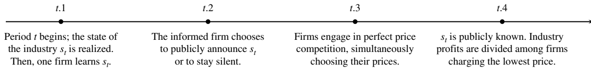
Figure 1 Model Timeline
